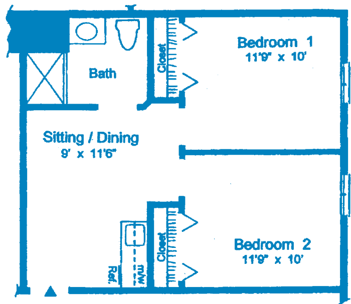
Two Bedroom Apartment (typical) 390 Sq. Ft. (Approx.)
